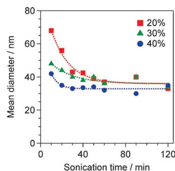
Figure 2. Mean diameters of the GaNPs as a function of ultrasonication time for different ultrasonication powers at 20°C. The dashed lines correspond to monoexponential fitting curves.
